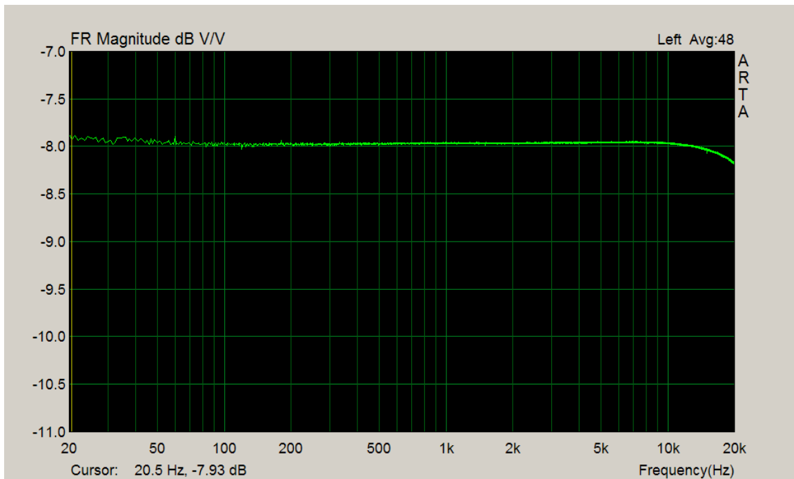
Frequency response at 1 watt output
